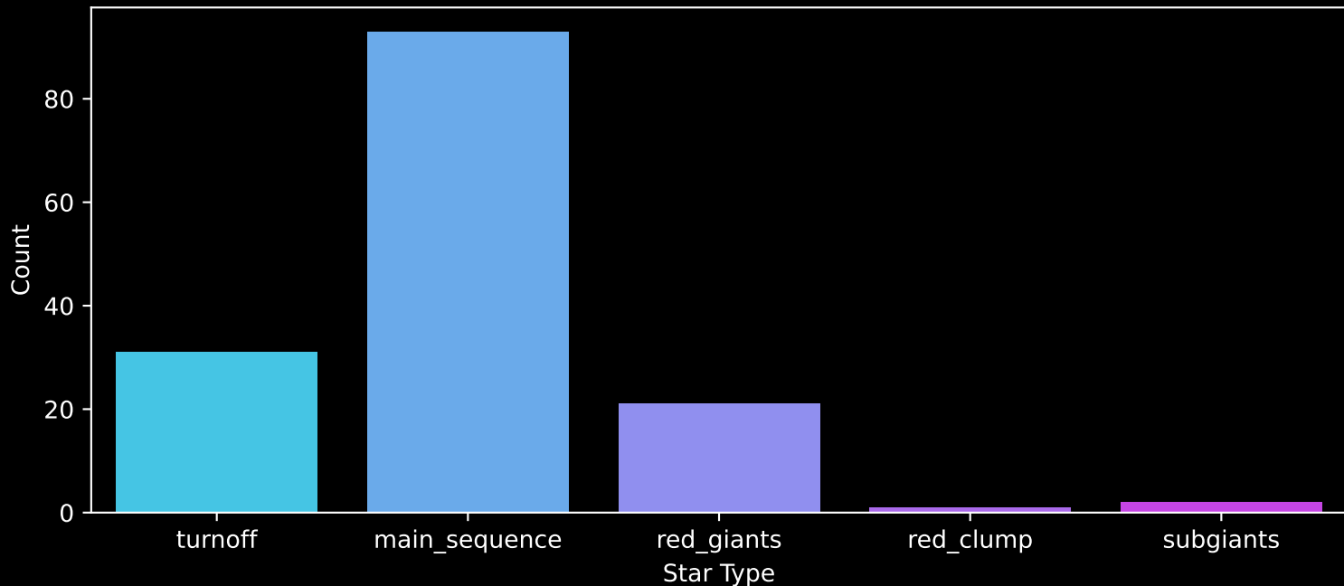
APOGEE DR17 Field: [045+56_MGA] Count plot of Star Type
