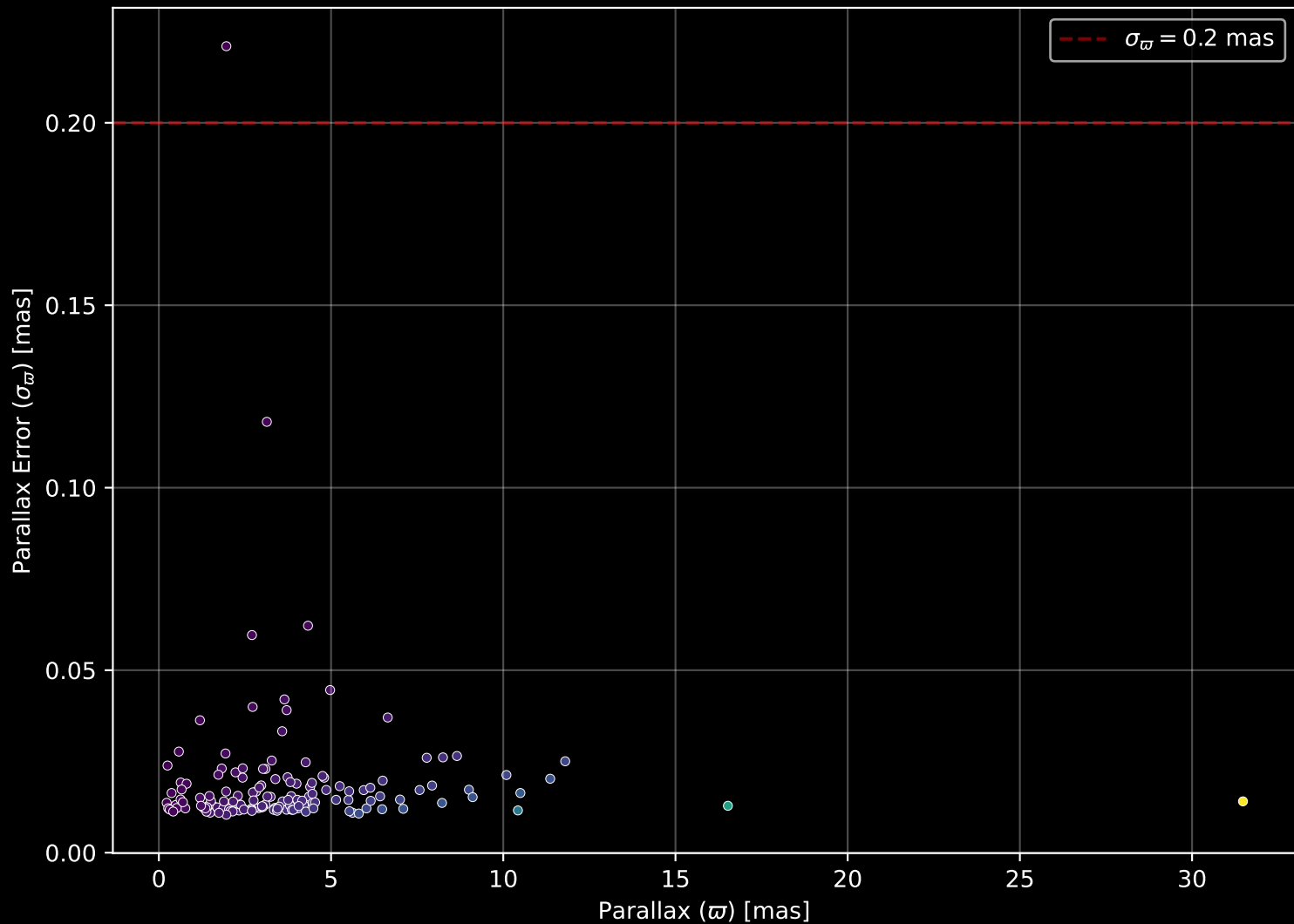
APOGEE DR17 Field: [045+56_MGA] Parallax Quality (n= 148)
