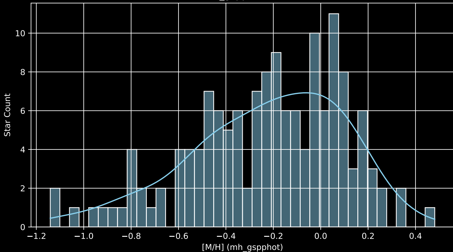
APOGEE DR17 Field: [045+56_MGA [M/H] (mh_gspphot) (n= 146)
