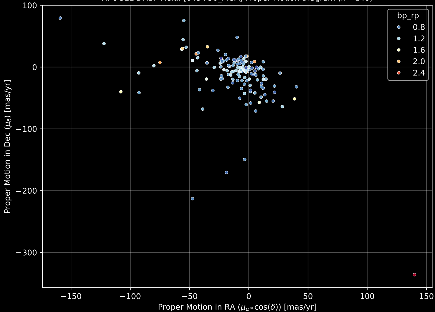
APOGEE DR17 Field: [045+56_MGA] Proper Motion Diagram (n= 148)
