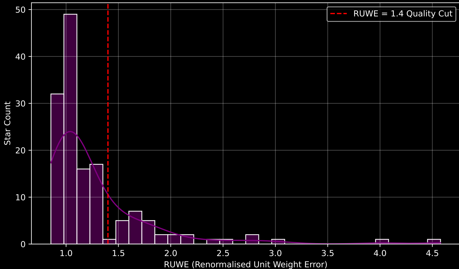
GAPOGEE DR17 Field [045+56_MGA] RUWE Distribution (n= 145)
